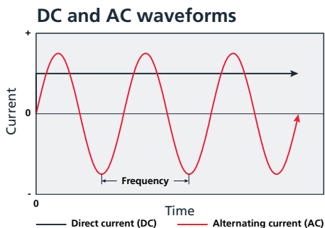
Figure 5-12: Direct currents are constant with respect to time while alternating currents are time-dependent waveforms with a frequency component. The frequency describes the number of complete cycles per second.
