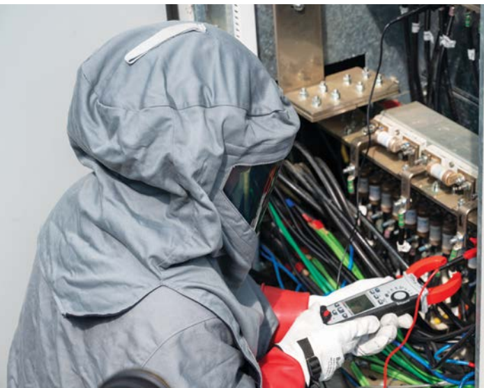
Figure 5-18: PV systems can operate at dangerously high amperages. Technicians should be aware of the risks associated with the expected system current and voltage, and should wear appropriate PPE.
