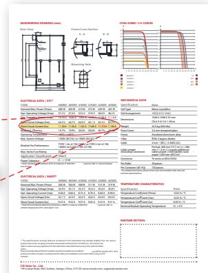
Figure 5-11: The I_{sc} value provided in the module datasheet can be recalculated with onsite irradiance data.
