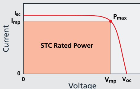
I-V curve at STC Figure 5-9
