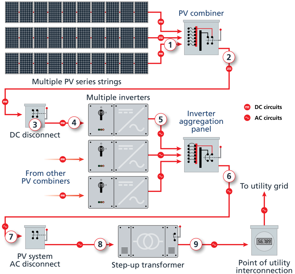
Figure 5-14: Amperage measurements are taken at multiple locations within the PV array and on the utility side of the inverter.
