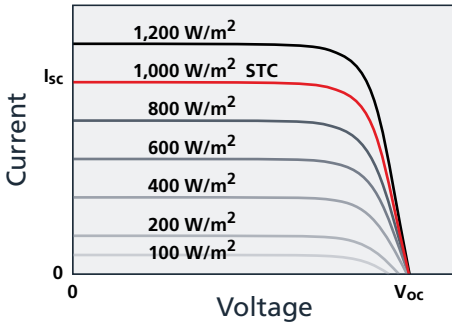
Figure 5-10: A module's I_{sc} is directly proportional to the intensity of sunlight on the module. Note that module current may rise above the I_{sc} value listed on the data sheet, which was measured at STC.
