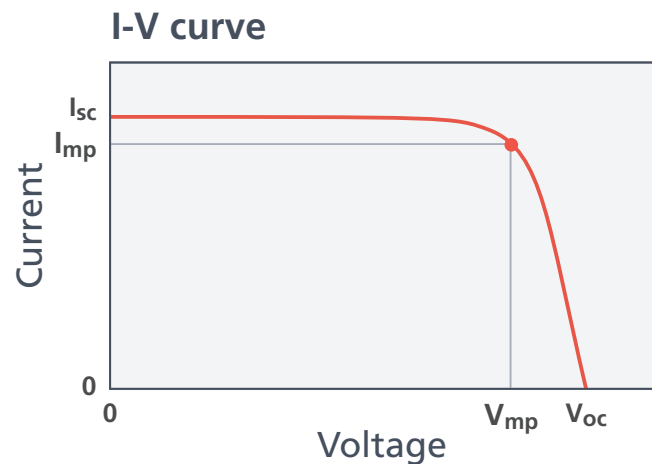
Figure 4-5: A typical PV module I-V curve. The open-circuit voltage (VOC) is the point on the curve with the maximum voltage value and zero current.
