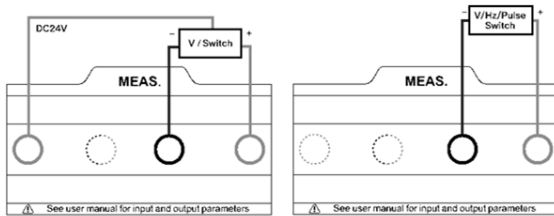
Figure 6 Voltage / Frequency / Pulse / Switch Measurement
