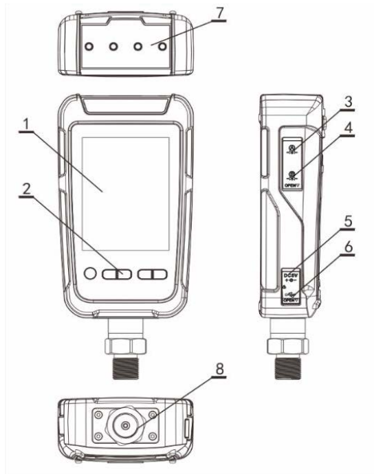
Figure 1 Basic Structure
