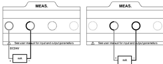
Figure 7 Current Measurement
