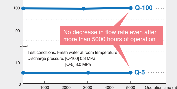
Changes in flow rate over continuous operation
